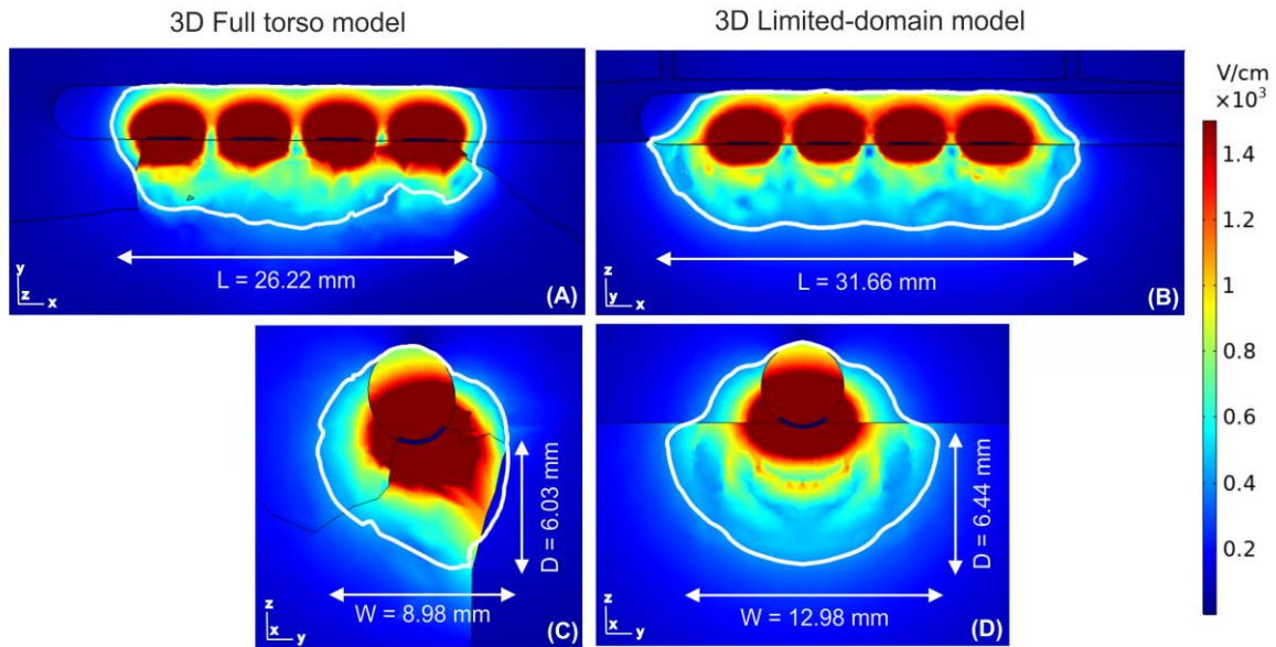
Figure 7 Electric field distributions on planes XY (A,B) and YZ (C,D) around the electrodes computed from the 3D full torso (A,C) and the 3D limited-domain model (B,D) (both with the same scale). The white contour corresponds to the 400 V/cm electric field isoline.
