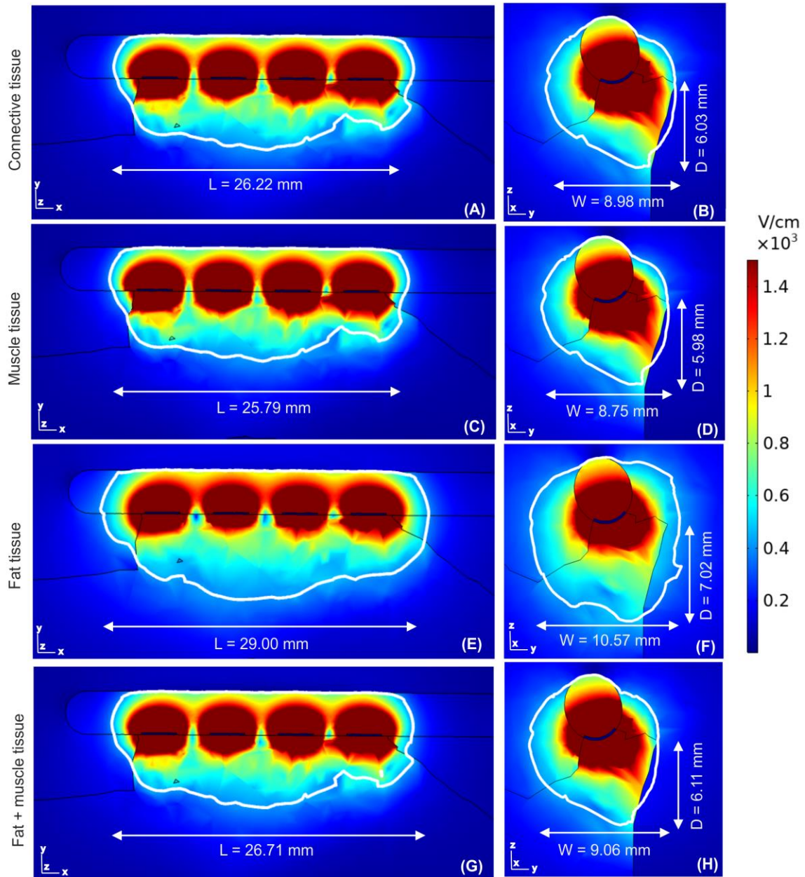
Figure 5 Electric field distributions around the electrodes corresponding with the longitudinal axis ( A,C,E,G ) and transverse through the middle point of the third electrode ( B,D,F,H ) for different types of tissue surrounding the organs: connective ( A,B ), muscle ( C,D ), fat ( E,F ) and mixture of fat and muscle ( G,H ). The white contour corresponds to the 400 V/cm electric field isoline.
