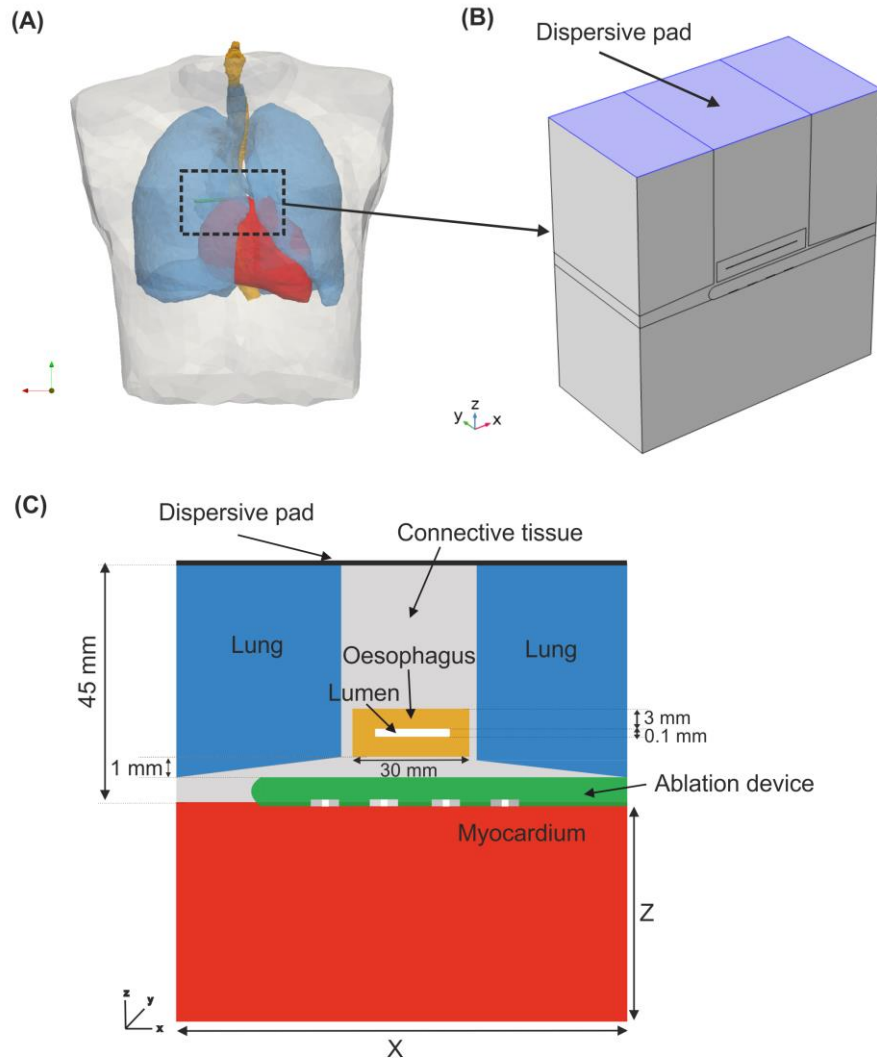
Figure 2 Geometry of the 3D limited-domain model (B) which only considers a fragment of the region of interest corresponding with the full torso (A) . The dispersive pad in the limited-domain model is placed on the top surface of the model (B and C) .
